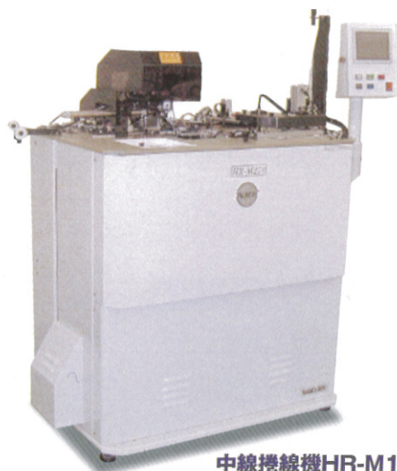
中線捲線機HR-M170/270 Medium fine coil winder HR-M170/270
